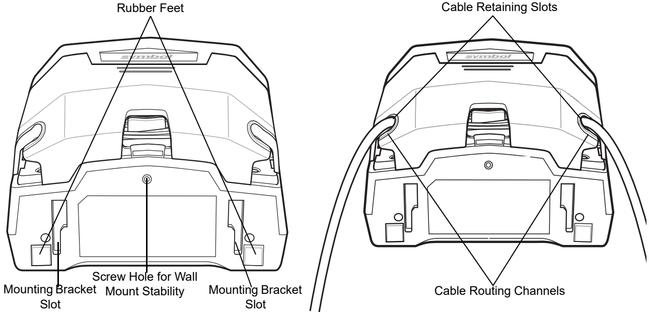
Figure 1-3 DS7708 Views - Bottom and With and Without Cables
