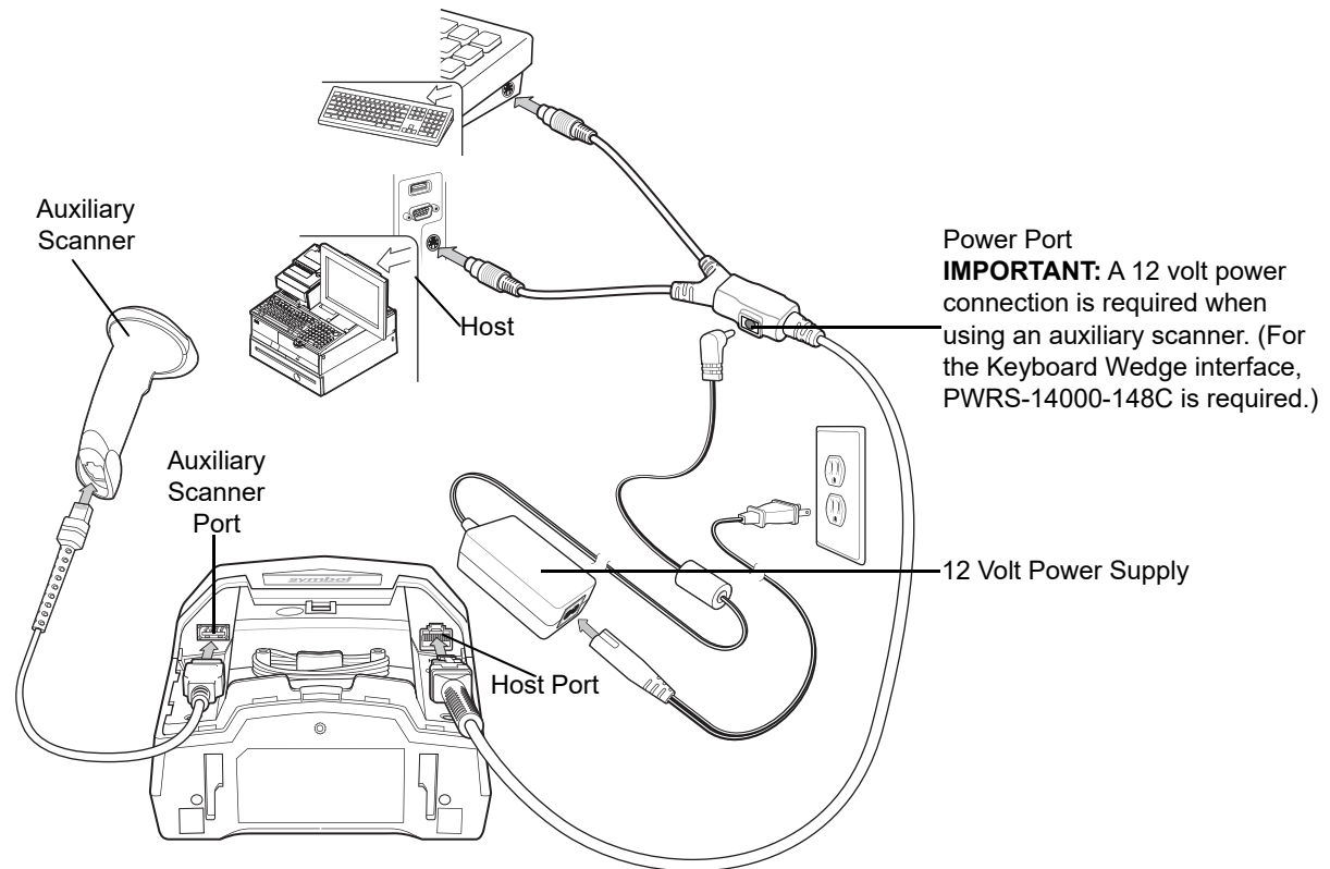
Figure 9-2 Keyboard Wedge Connection - With Auxiliary Scanner/Power Supplied Externally
